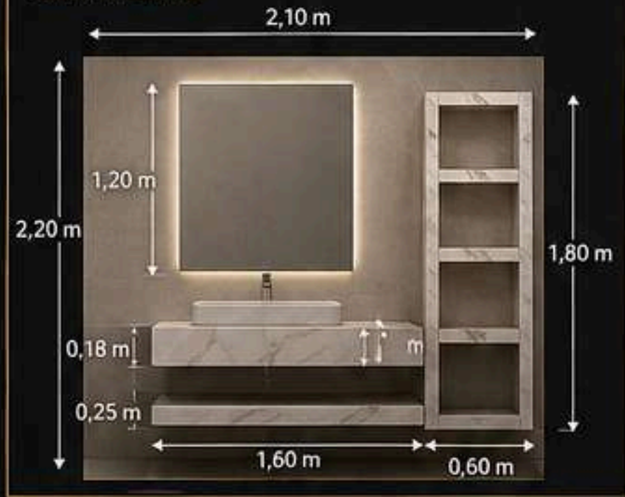
VISTA FRONTAL
